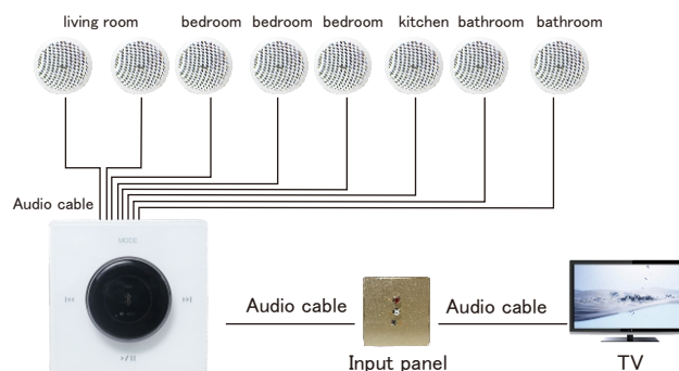
Wall amplifier
